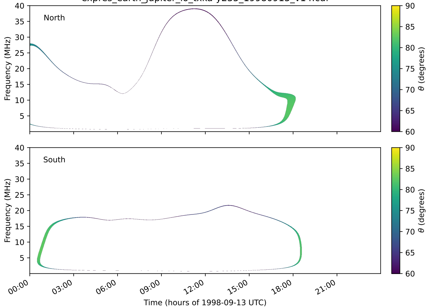
expres_earth_jupiter_io_txka-y235_19980913_v14.cdf
