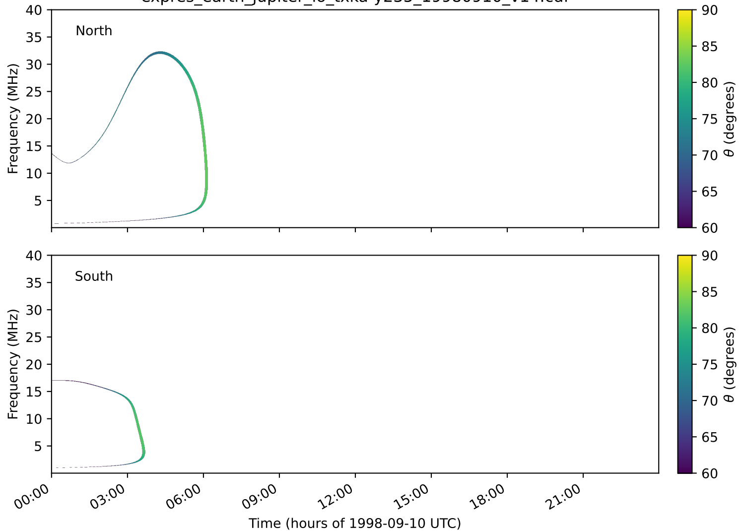
expres_earth_jupiter_io_txka-y235_19980910_v14.cdf
