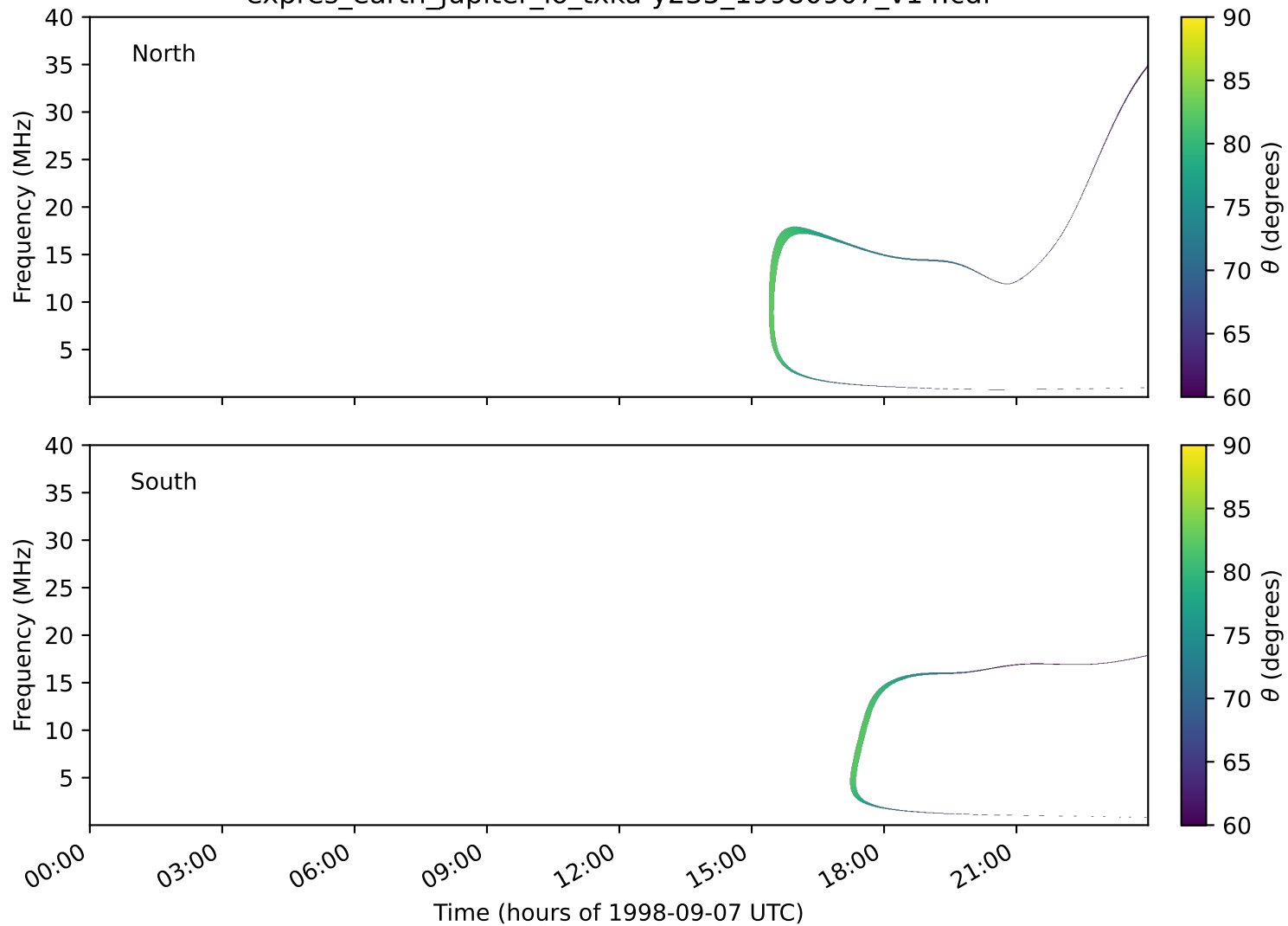
expres_earth_jupiter_io_txka-y235_19980907_v14.cdf
