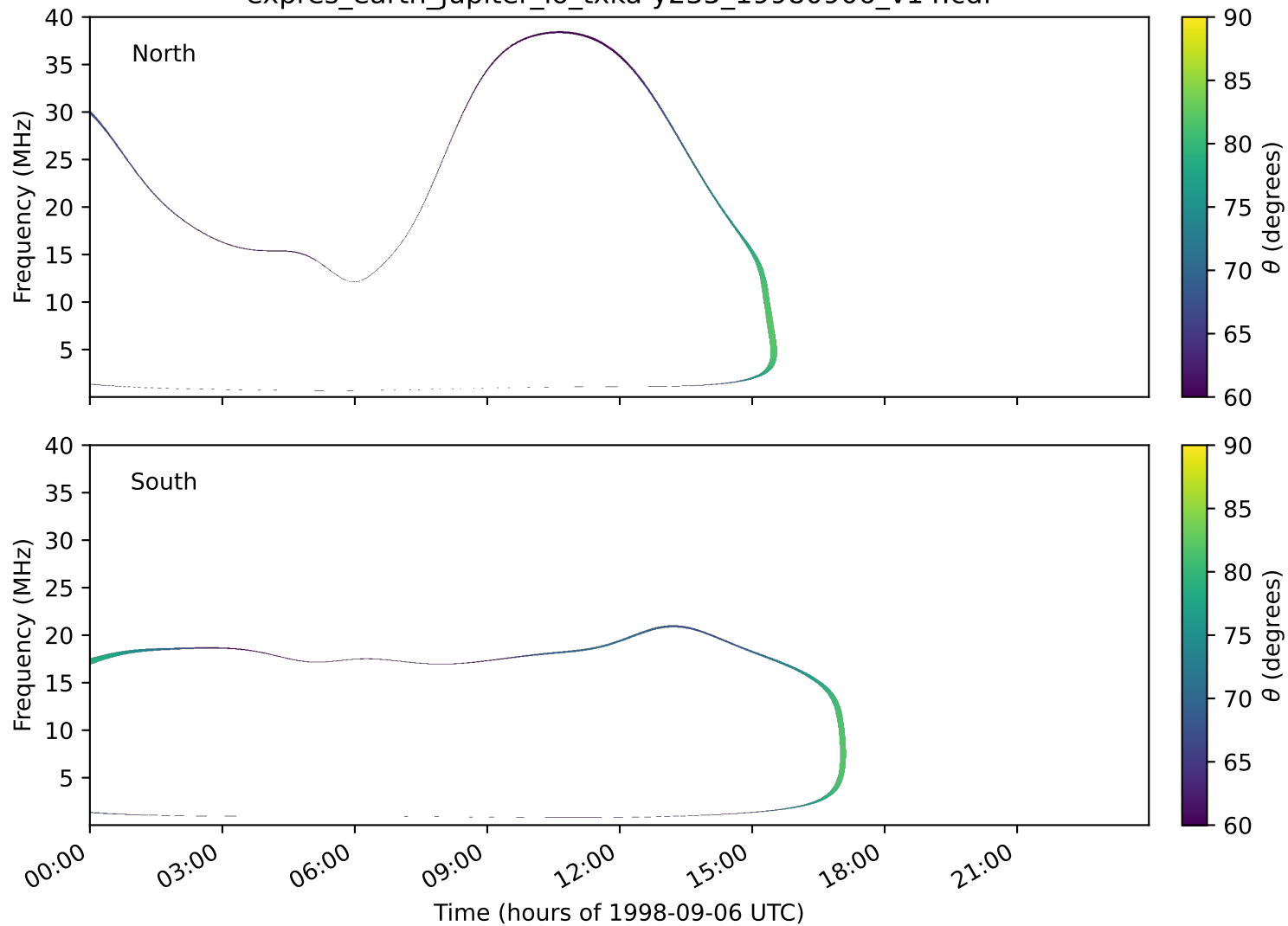
expres_earth_jupiter_io_txka-y235_19980906_v14.cdf
