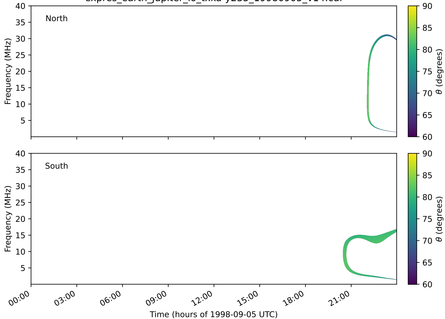
expres_earth_jupiter_io_txka-y235_19980905_v14.cdf
