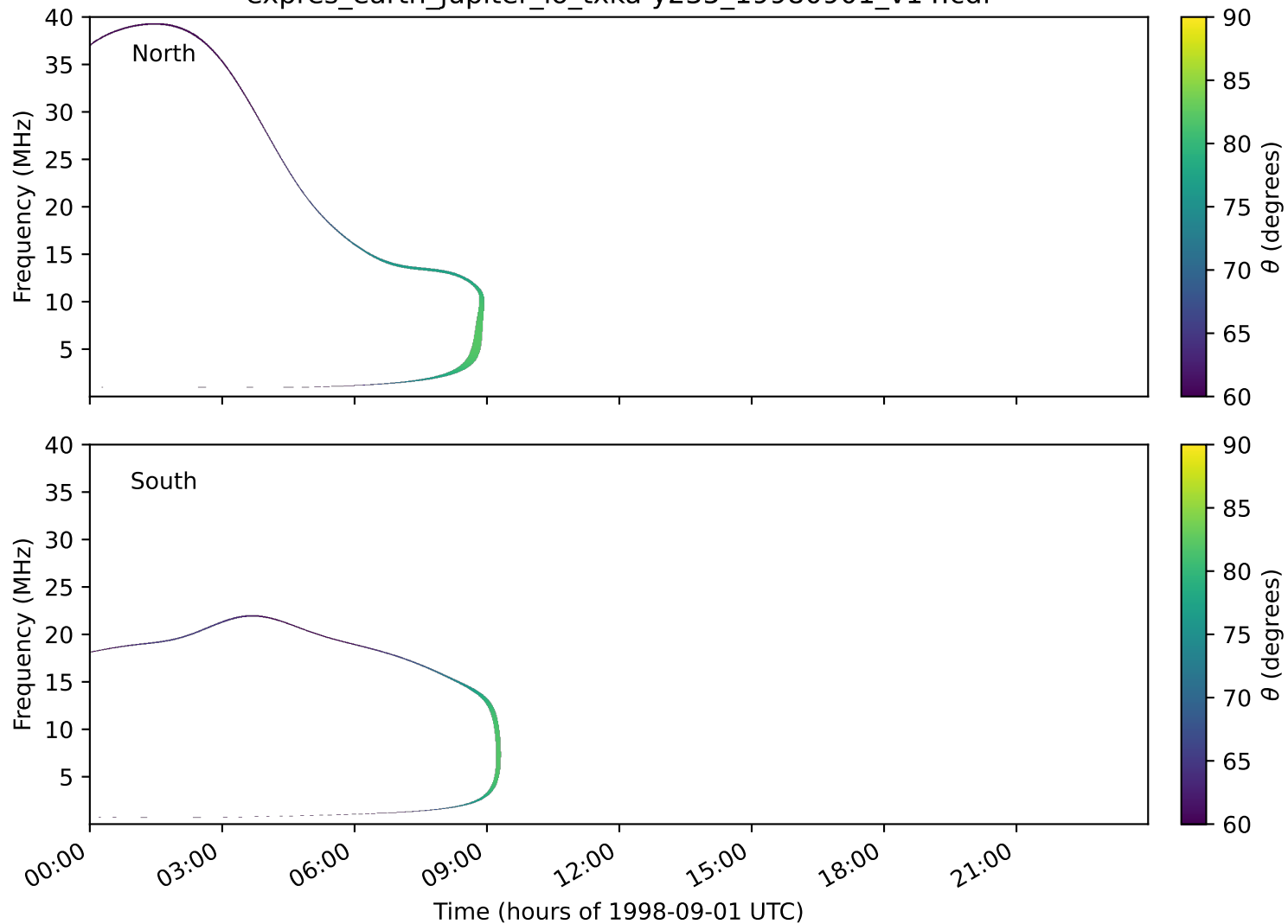
expres_earth_jupiter_io_txka-y235_19980901_v14.cdf
