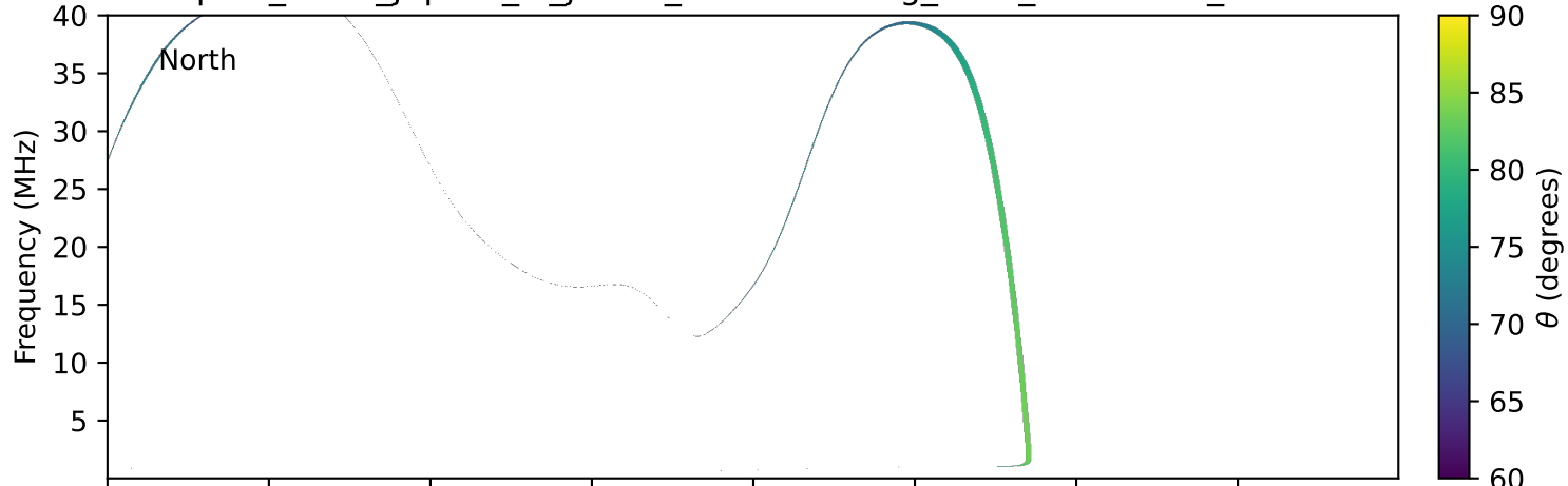
expres_earth_jupiter_io_jrm33_lossc-wid1deg_3kev_19980929_v11.cdf
