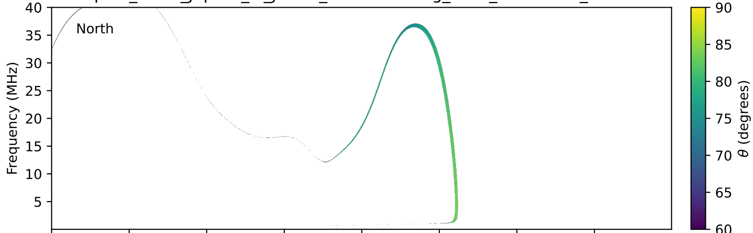
expres_earth_jupiter_io_jrm33_lossc-wid1deg_3kev_19980922_v11.cdf
