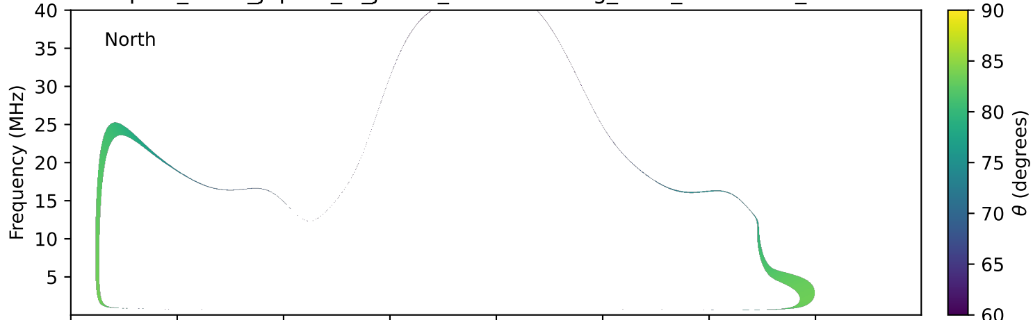
expres_earth_jupiter_io_jrm33_lossc-wid1deg_3kev_19980920_v11.cdf
