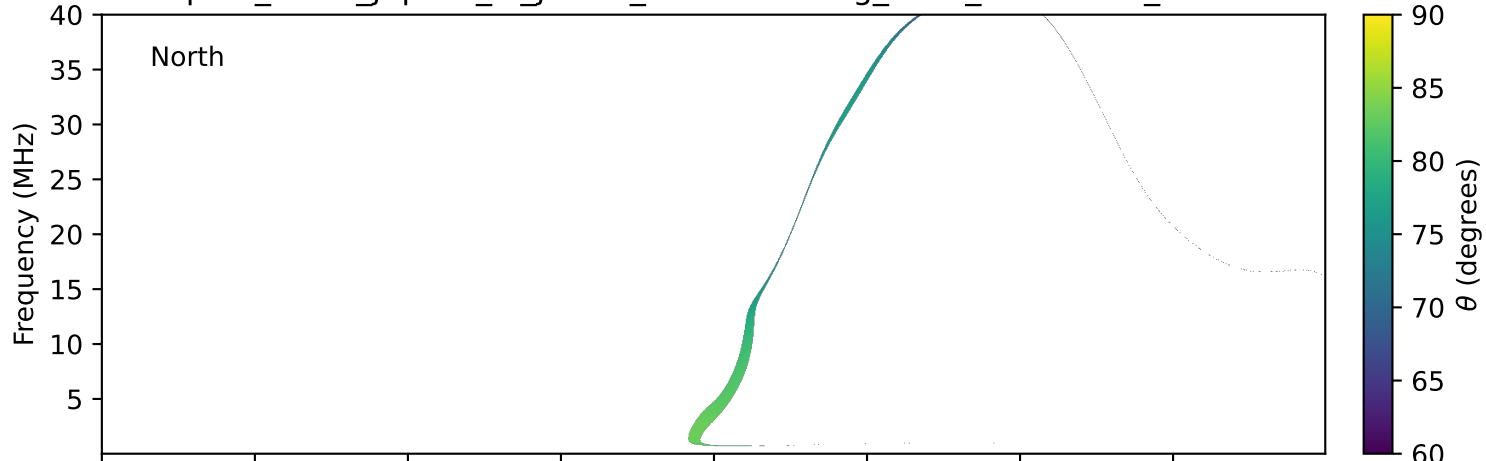
expres_earth_jupiter_io_jrm33_lossc-wid1deg_3kev_19980916_v11.cdf
