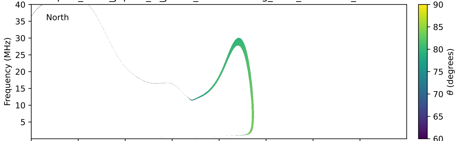
expres_earth_jupiter_io_jrm33_lossc-wid1deg_3kev_19980915_v11.cdf
