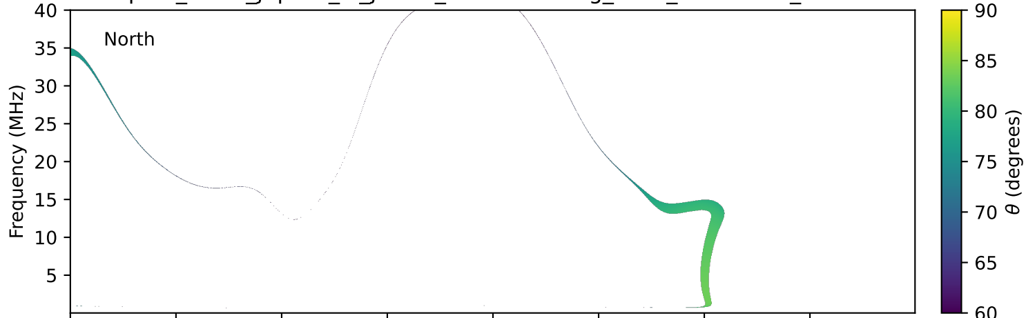
expres_earth_jupiter_io_jrm33_lossc-wid1deg_3kev_19980913_v11.cdf
