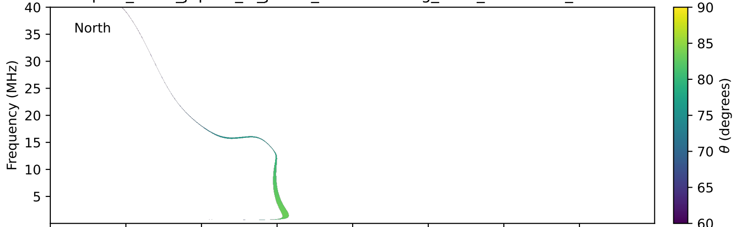
expres_earth_jupiter_io_jrm33_lossc-wid1deg_3kev_19980901_v11.cdf
