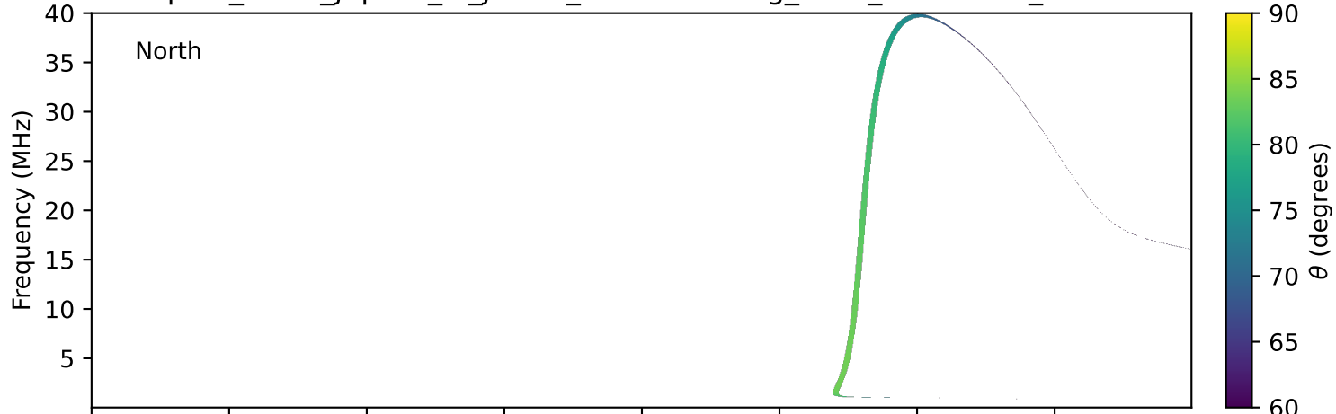
expres_earth_jupiter_io_jrm09_lossc-wid1deg_3kev_19980930_v11.cdf
