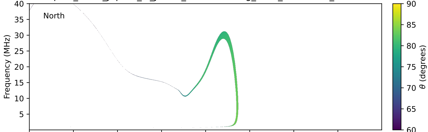
expres_earth_jupiter_io_jrm09_lossc-wid1deg_3kev_19980915_v11.cdf
