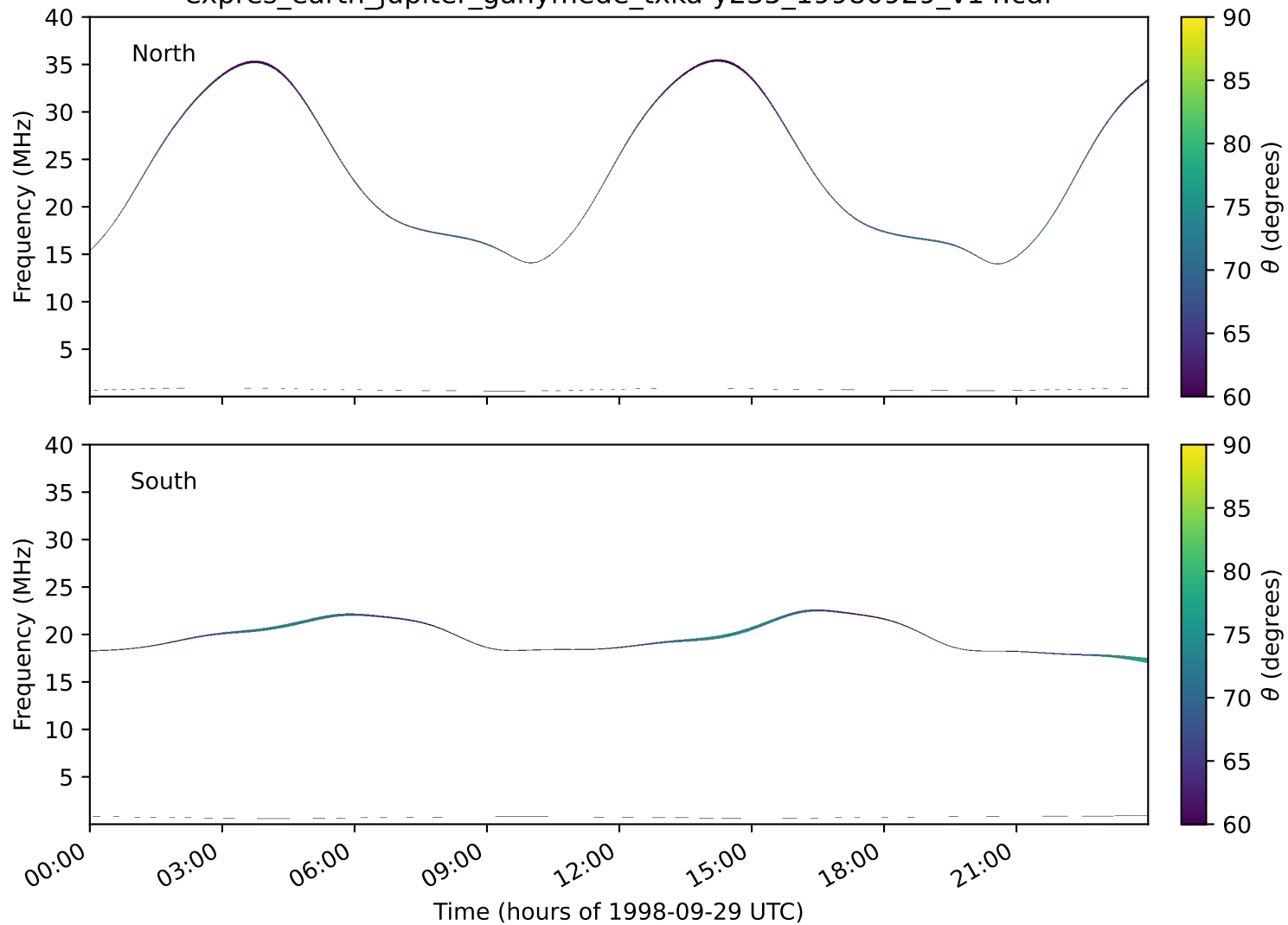
expres_earth_jupiter_ganymede_txka-y235_19980929_v14.cdf
