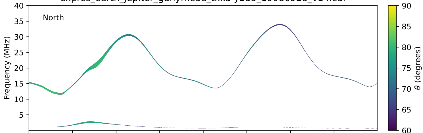
expres_earth_jupiter_ganymede_txka-y235_19980928_v14.cdf
