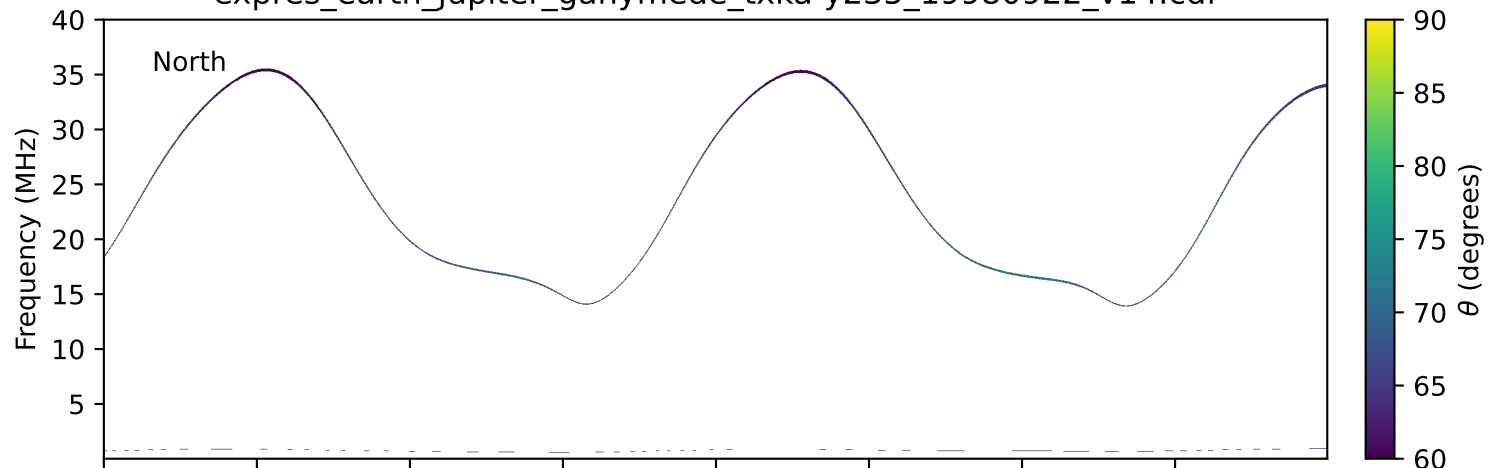
expres_earth_jupiter_ganymede_txka-y235_19980922_v14.cdf
