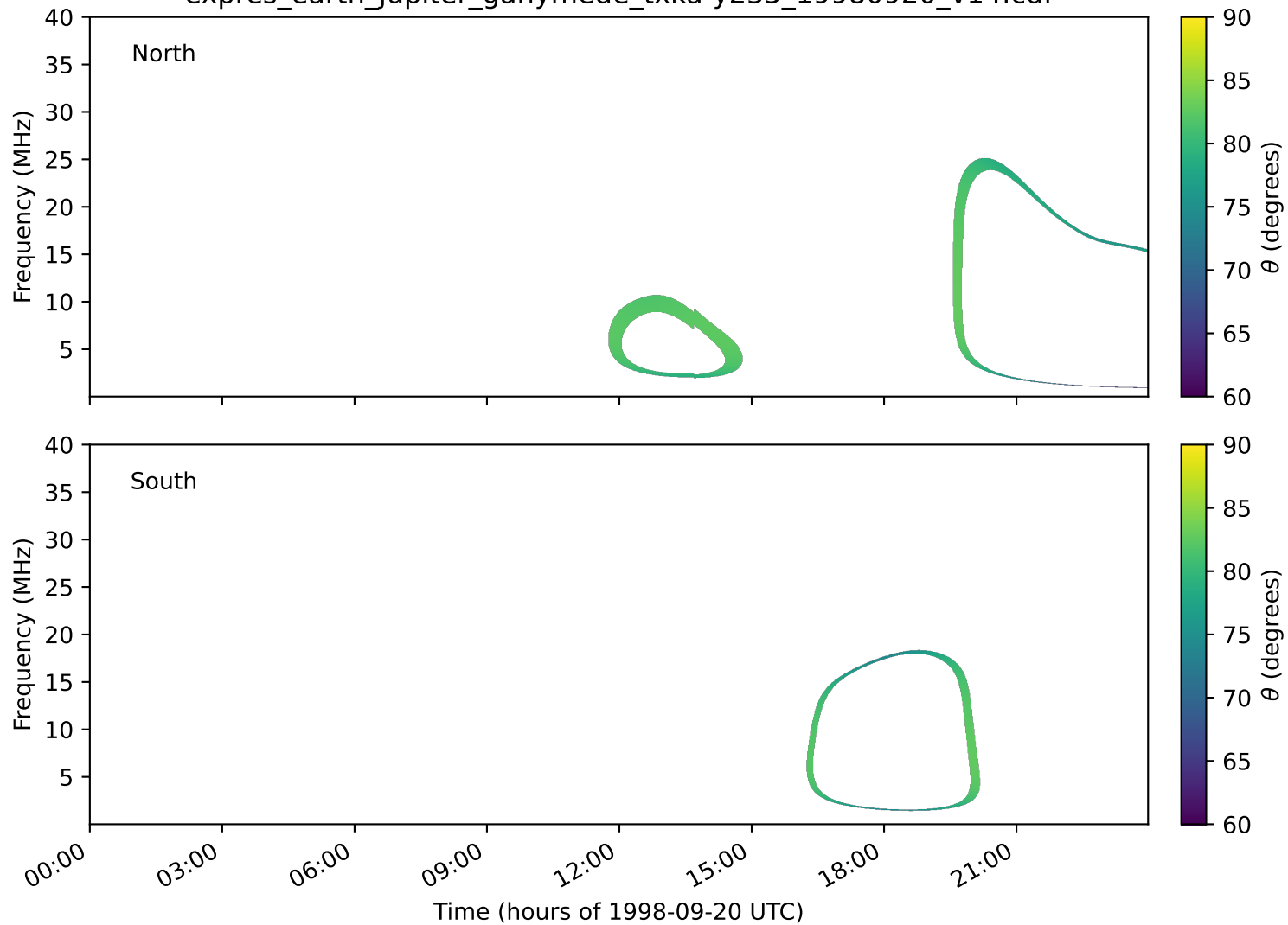
expres_earth_jupiter_ganymede_txka-y235_19980920_v14.cdf
