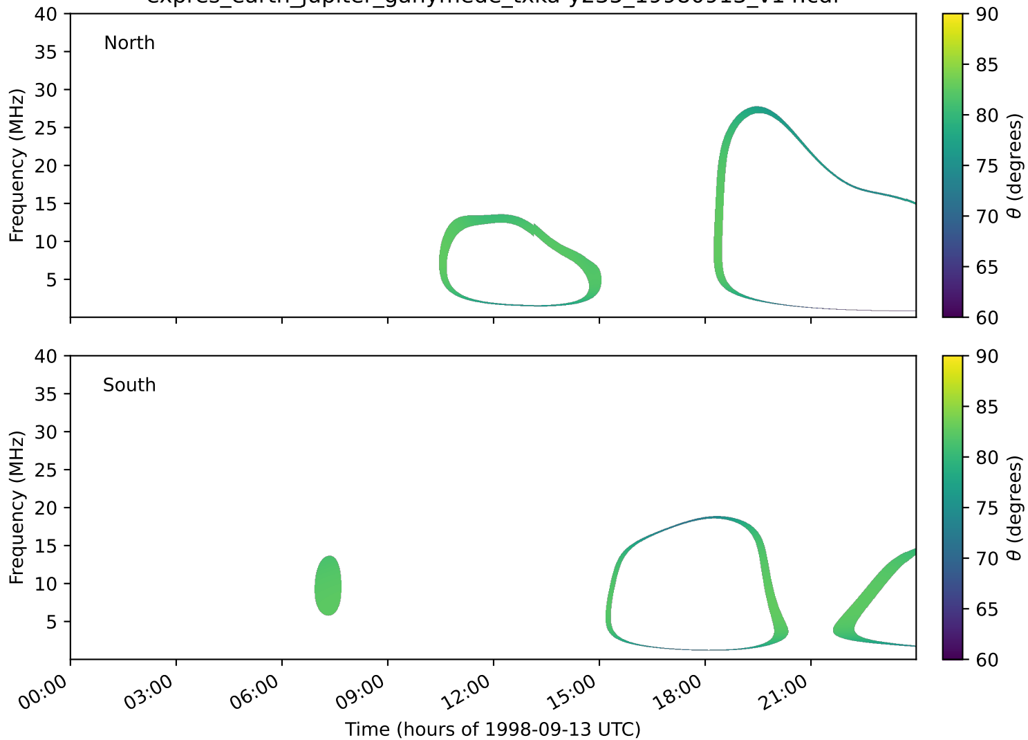
expres_earth_jupiter_ganymede_txka-y235_19980913_v14.cdf
