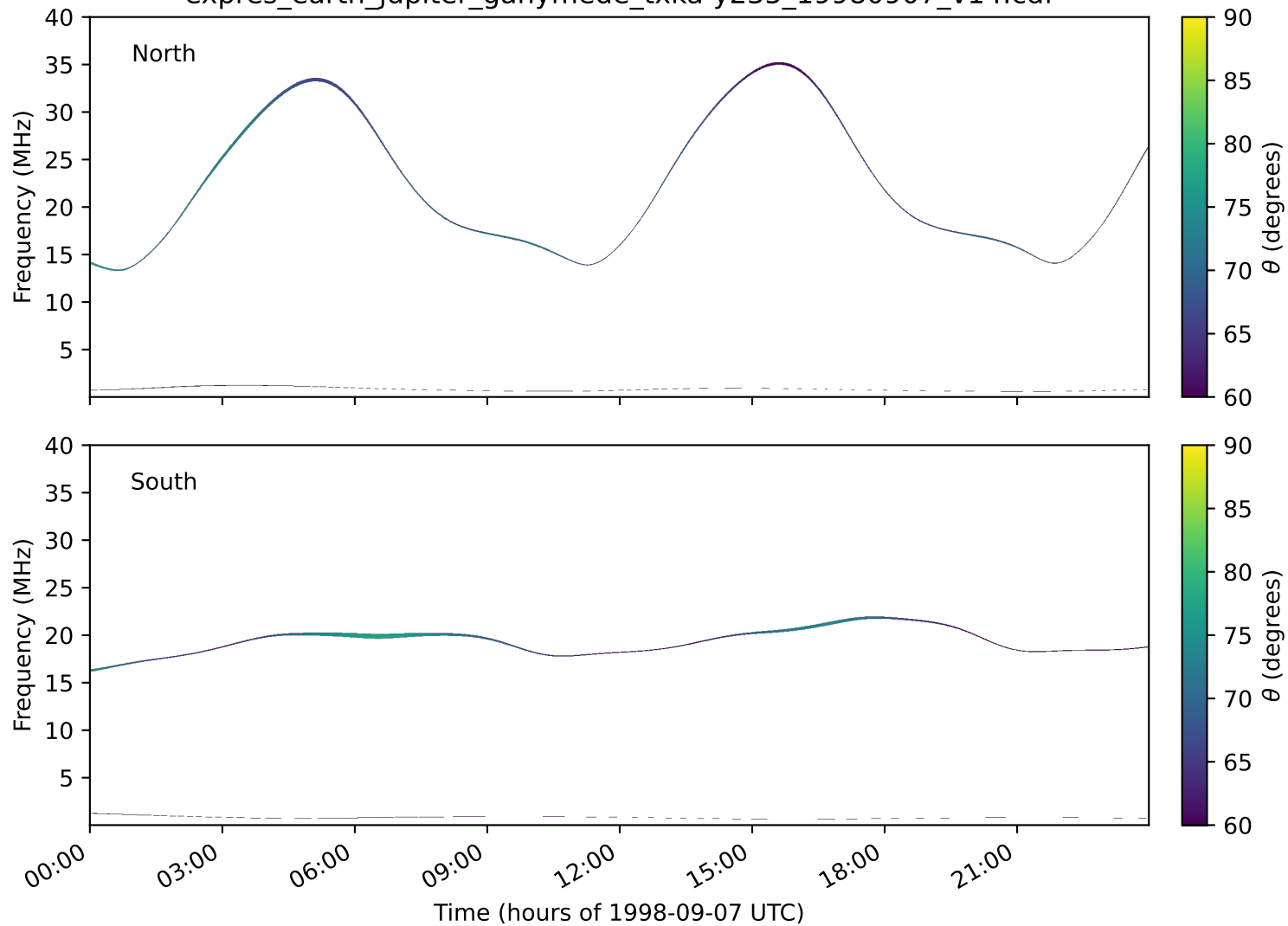
expres_earth_jupiter_ganymede_txka-y235_19980907_v14.cdf
