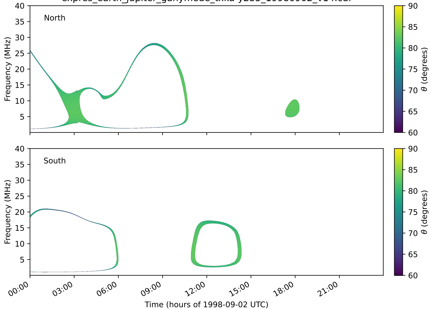
expres_earth_jupiter_ganymede_txka-y235_19980902_v14.cdf
