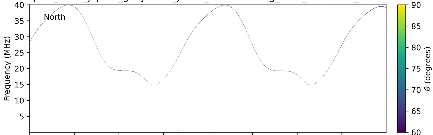
expres_earth_jupiter_ganymede_jrm33_lossc-wid1deg_3kev_19980915_v11.cdf
