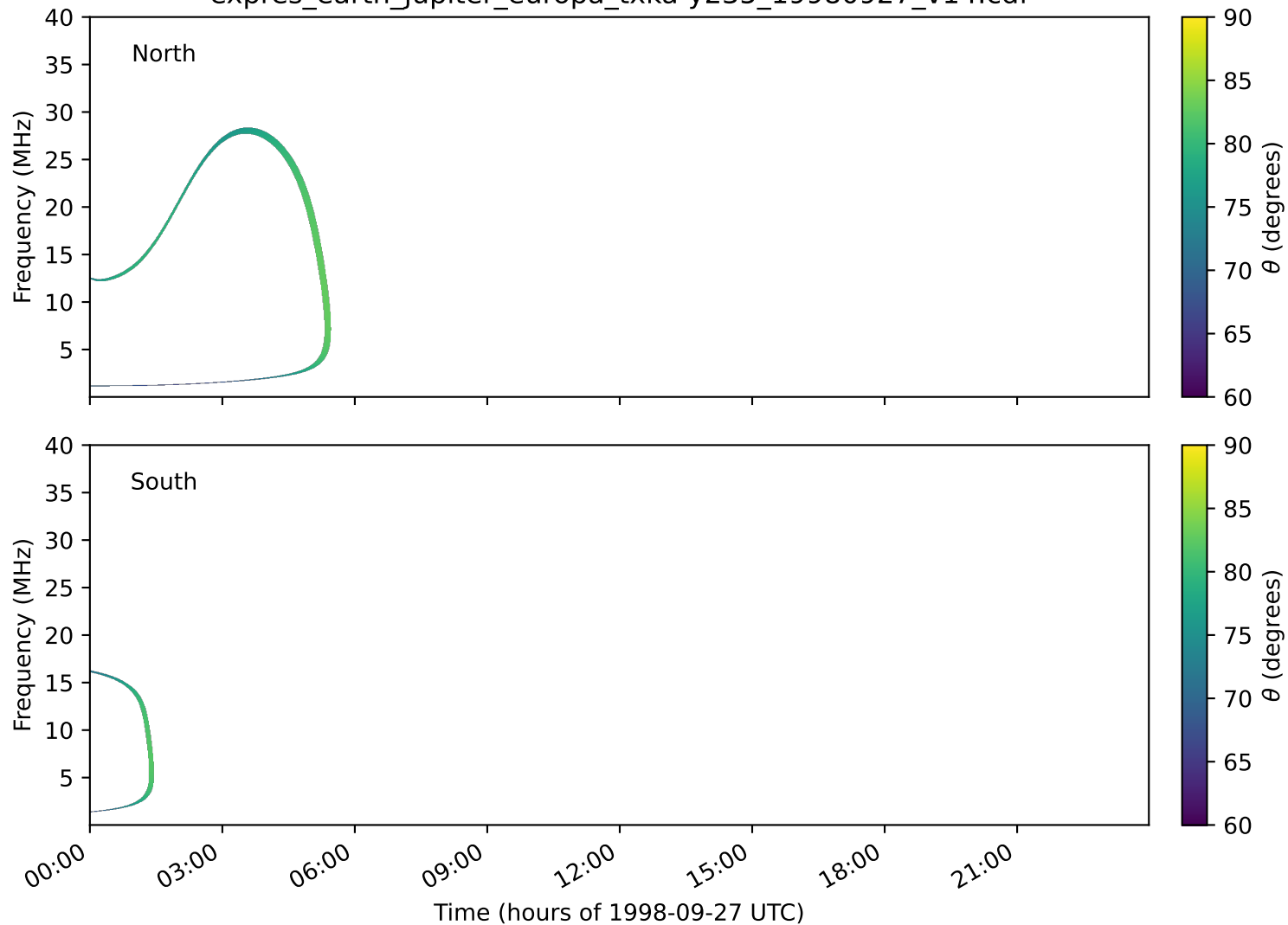
expres_earth_jupiter_europa_txka-y235_19980927_v14.cdf
