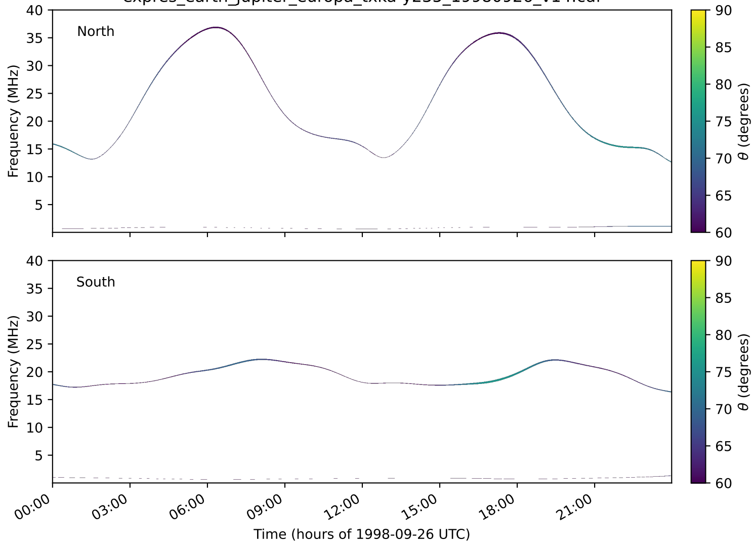
expres_earth_jupiter_europa_txka-y235_19980926_v14.cdf
