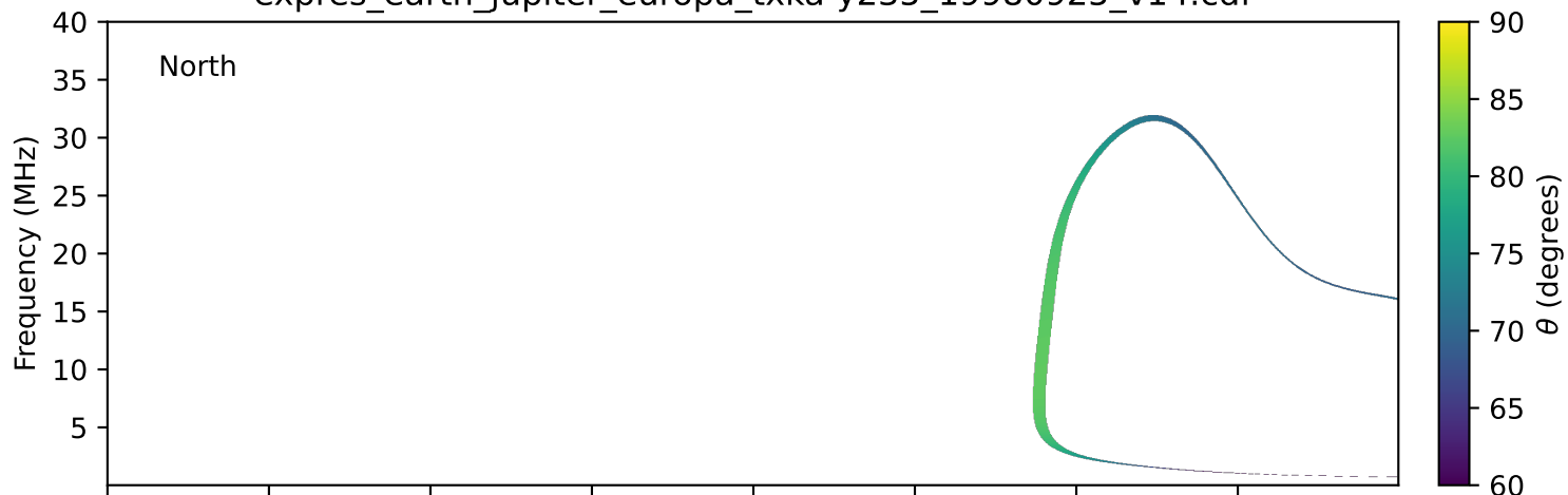
expres_earth_jupiter_europa_txka-y235_19980925_v14.cdf
