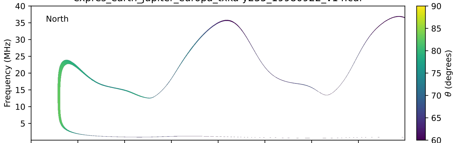
expres_earth_jupiter_europa_txka-y235_19980922_v14.cdf
