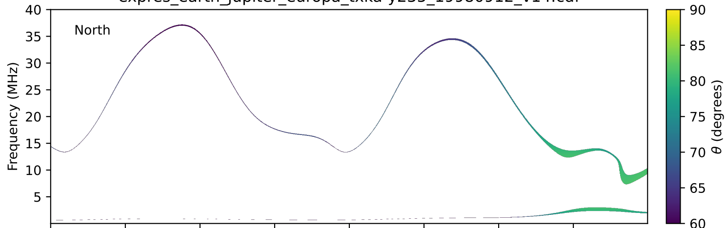
expres_earth_jupiter_europa_txka-y235_19980912_v14.cdf
