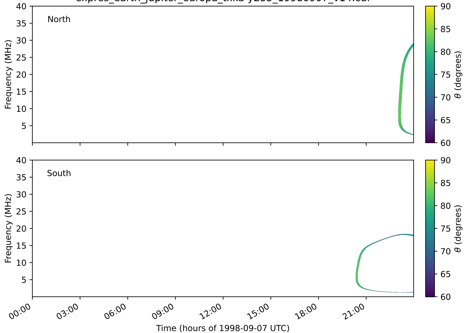
expres_earth_jupiter_europa_txka-y235_19980907_v14.cdf
