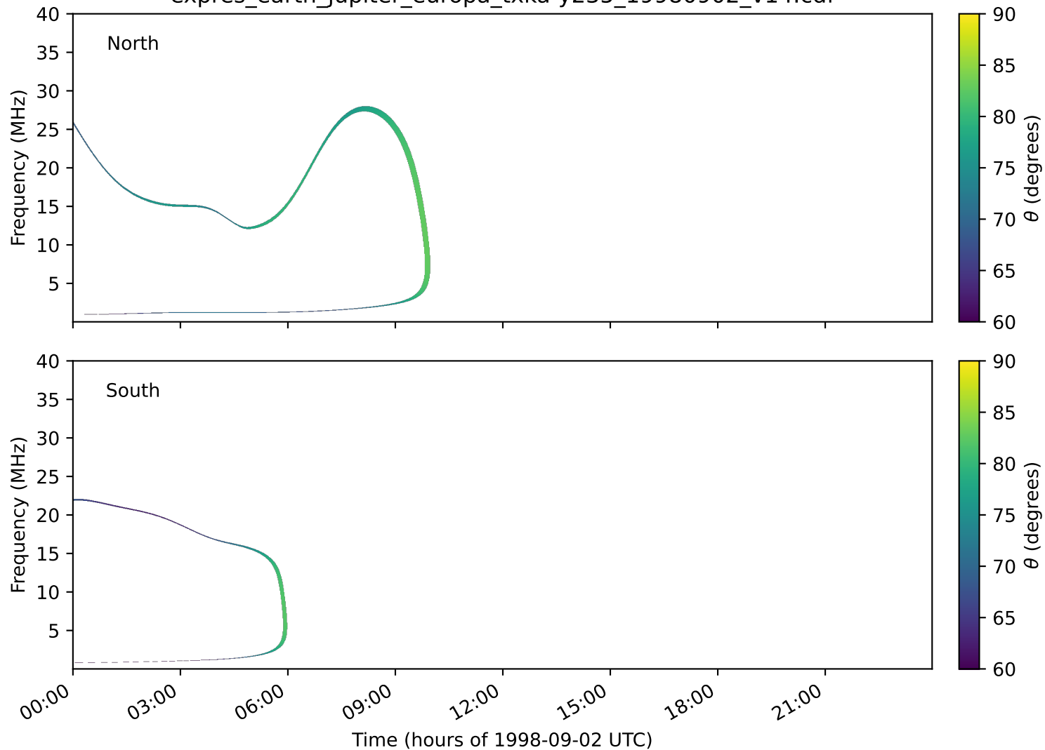
expres_earth_jupiter_europa_txka-y235_19980902_v14.cdf
