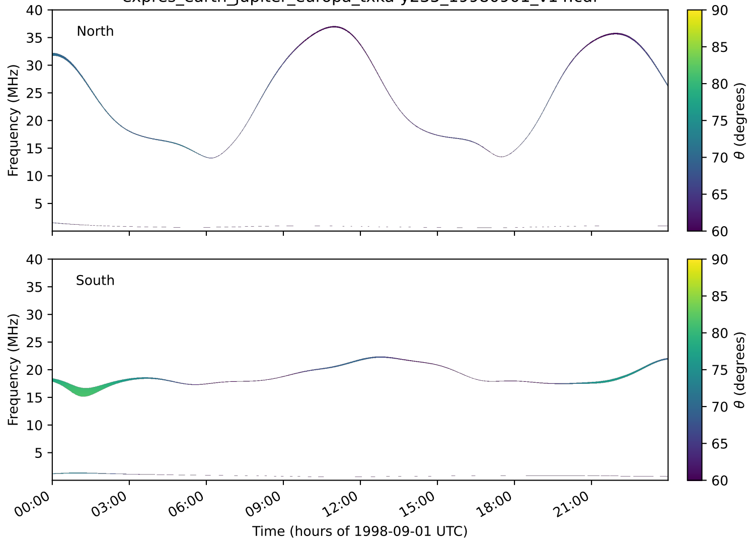
expres_earth_jupiter_europa_txka-y235_19980901_v14.cdf
