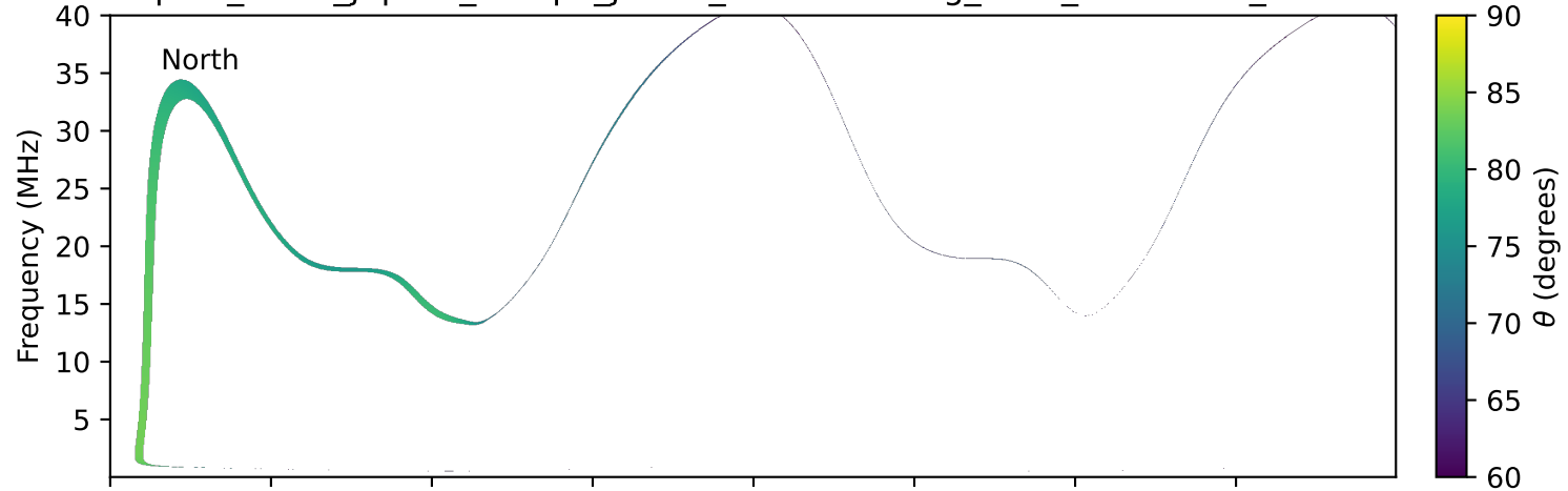
expres_earth_jupiter_europa_jrm33_lossc-wid1deg_3kev_19980915_v11.cdf
