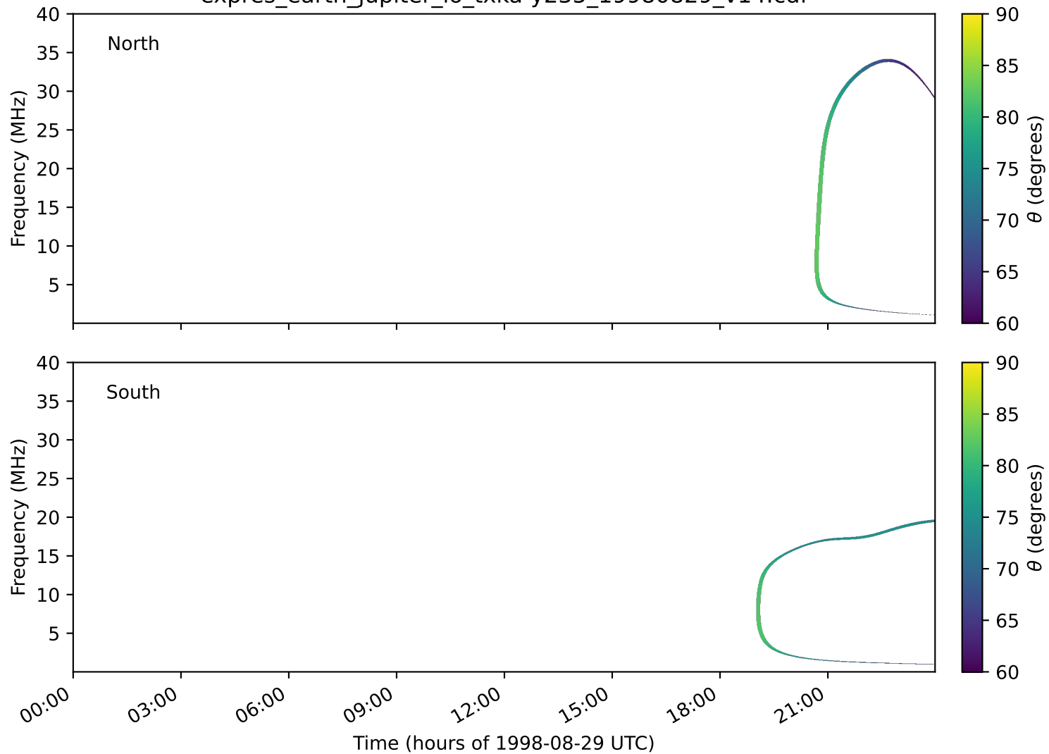
expres_earth_jupiter_io_txka-y235_19980829_v14.cdf
