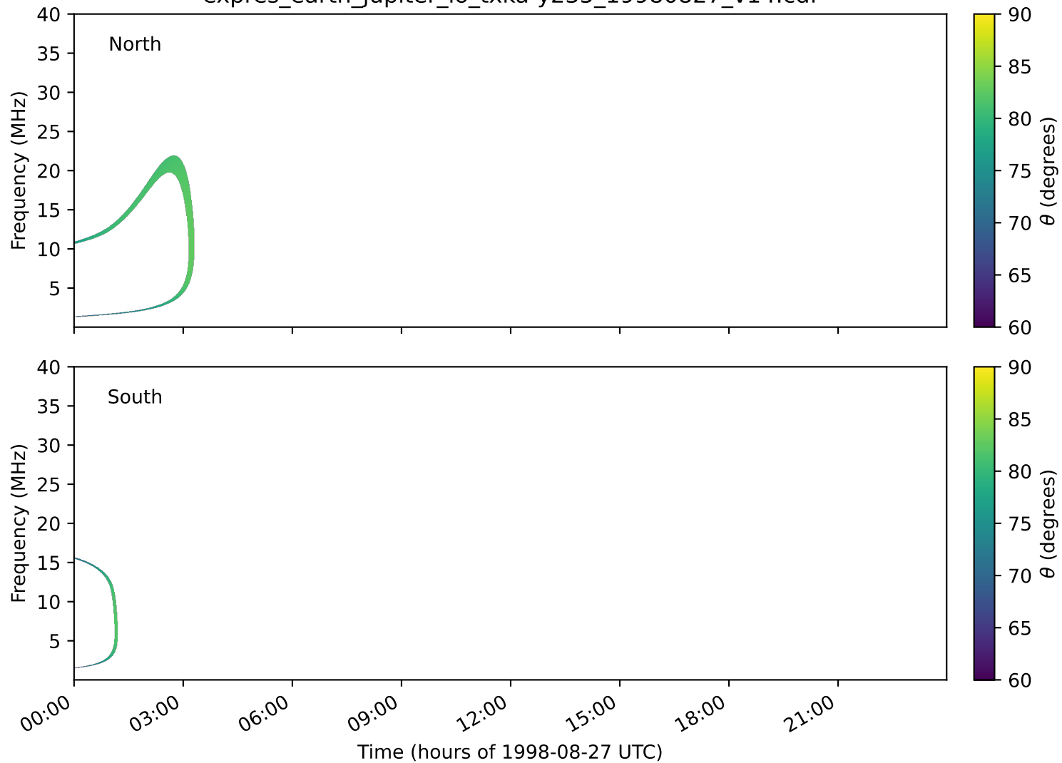
expres_earth_jupiter_io_txka-y235_19980827_v14.cdf
