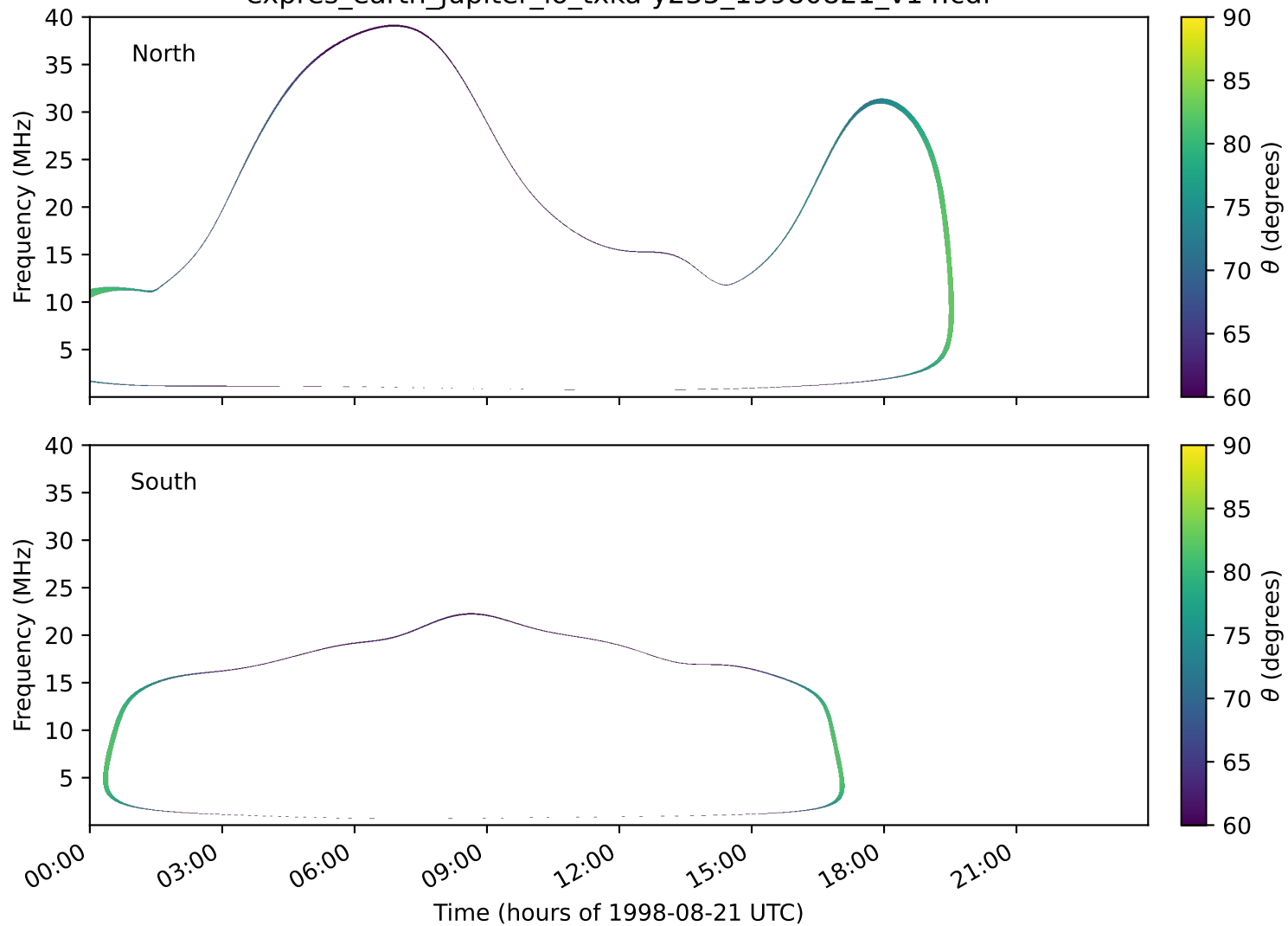
expres_earth_jupiter_io_txka-y235_19980821_v14.cdf
