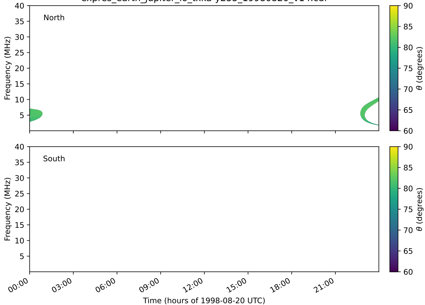
expres_earth_jupiter_io_txka-y235_19980820_v14.cdf
