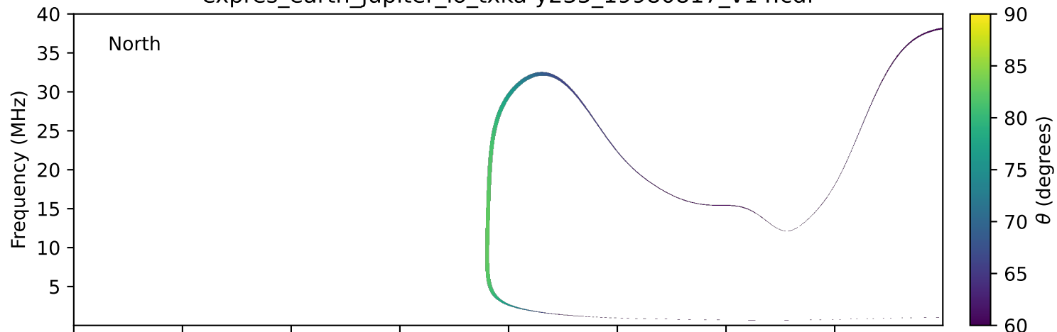
expres_earth_jupiter_io_txka-y235_19980817_v14.cdf
