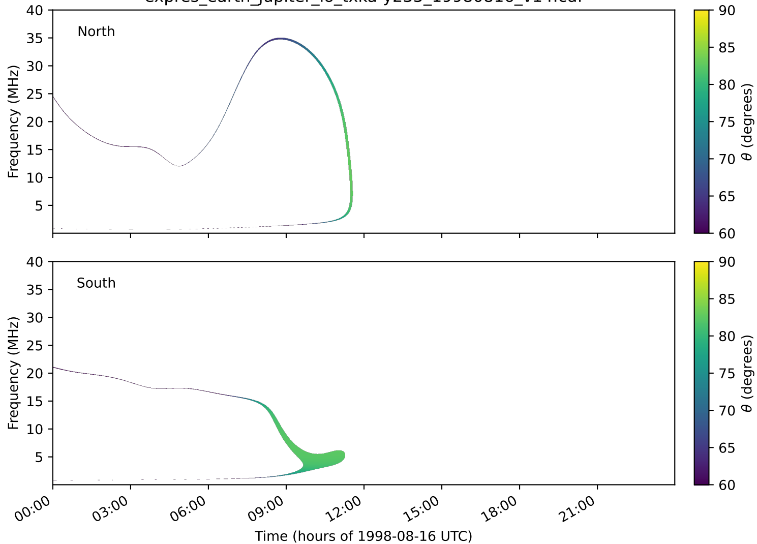
expres_earth_jupiter_io_txka-y235_19980816_v14.cdf
