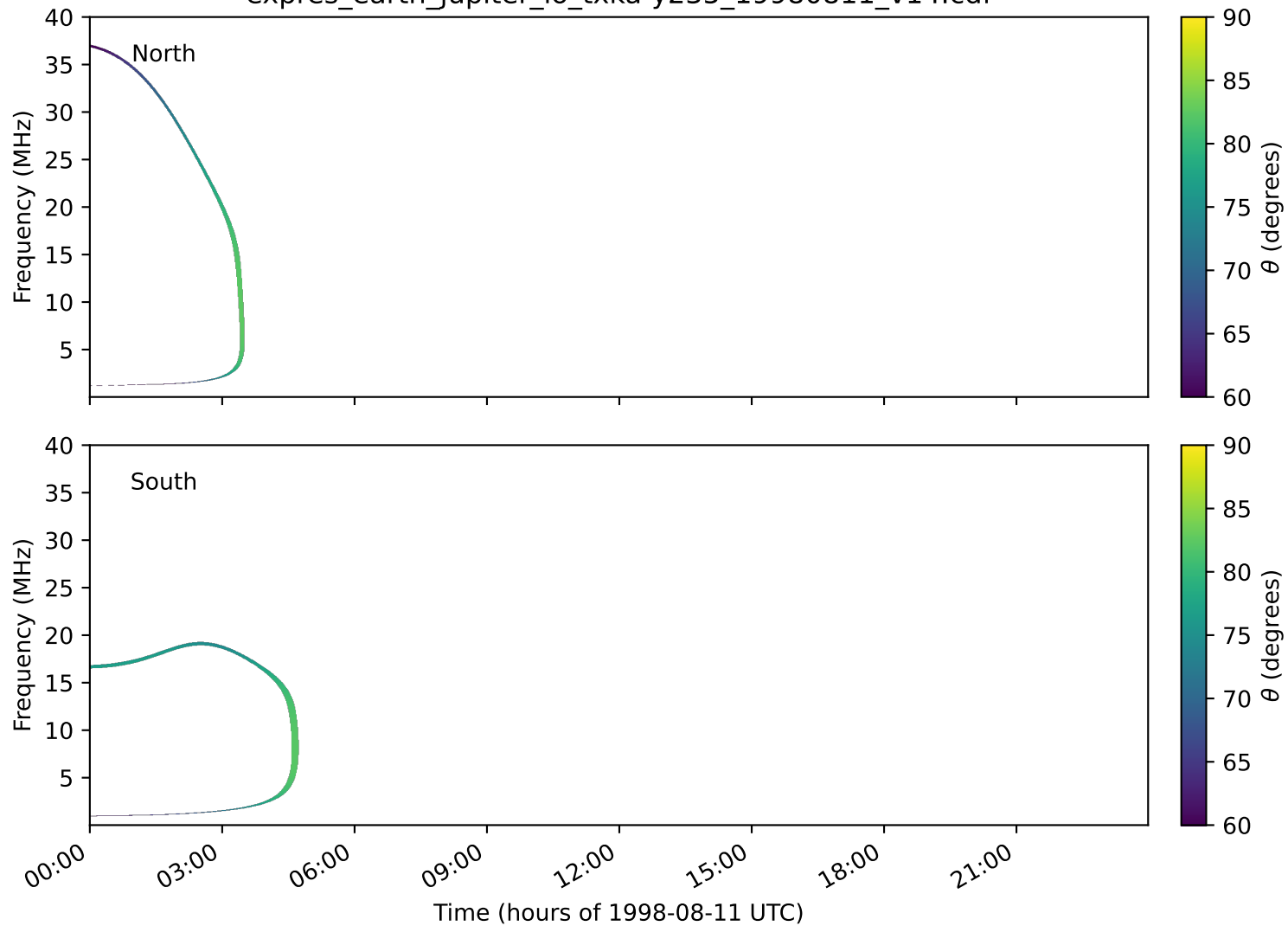
expres_earth_jupiter_io_txka-y235_19980811_v14.cdf
