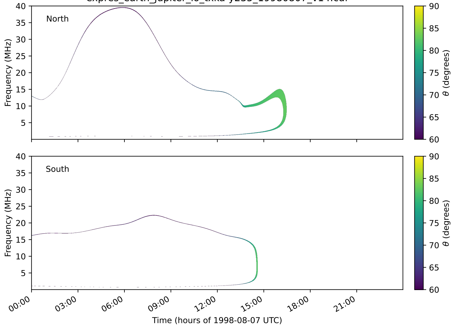
expres_earth_jupiter_io_txka-y235_19980807_v14.cdf
