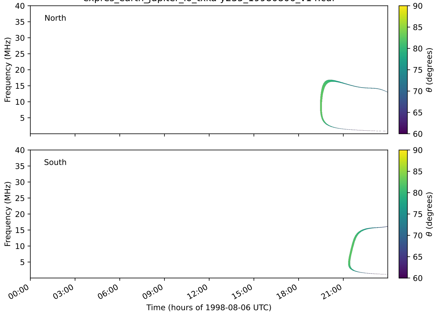
expres_earth_jupiter_io_txka-y235_19980806_v14.cdf
