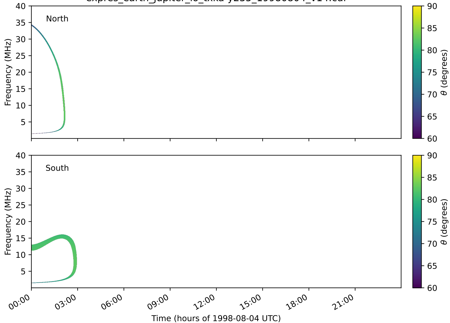
expres_earth_jupiter_io_txka-y235_19980804_v14.cdf
