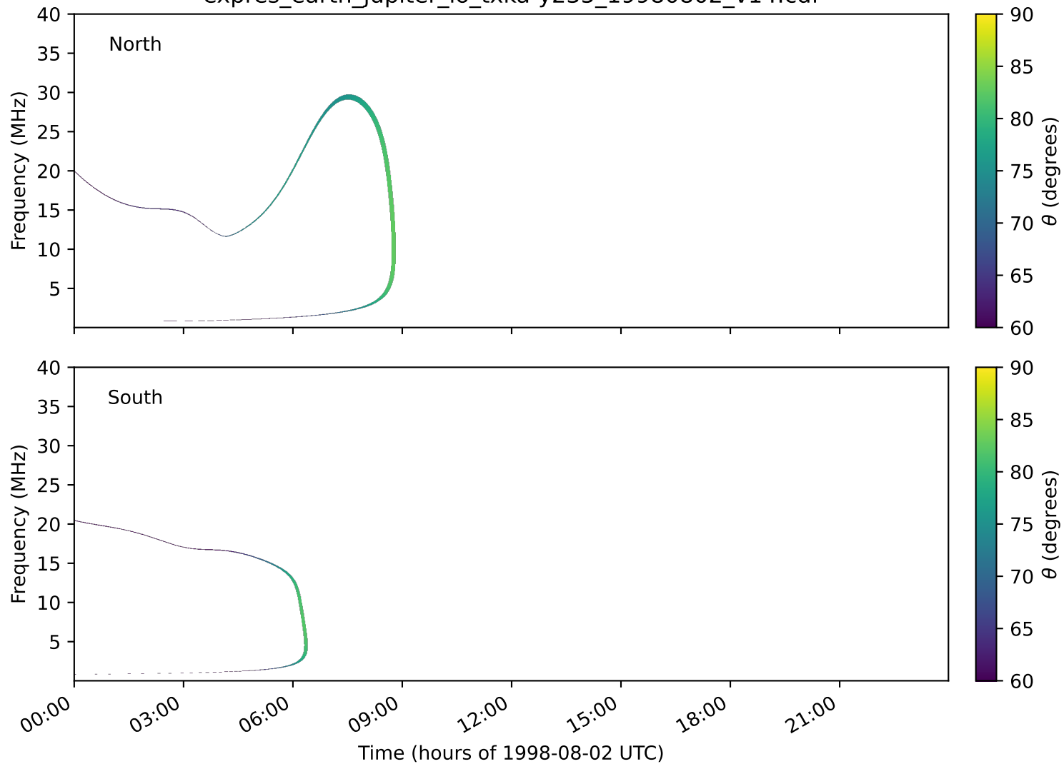
expres_earth_jupiter_io_txka-y235_19980802_v14.cdf
