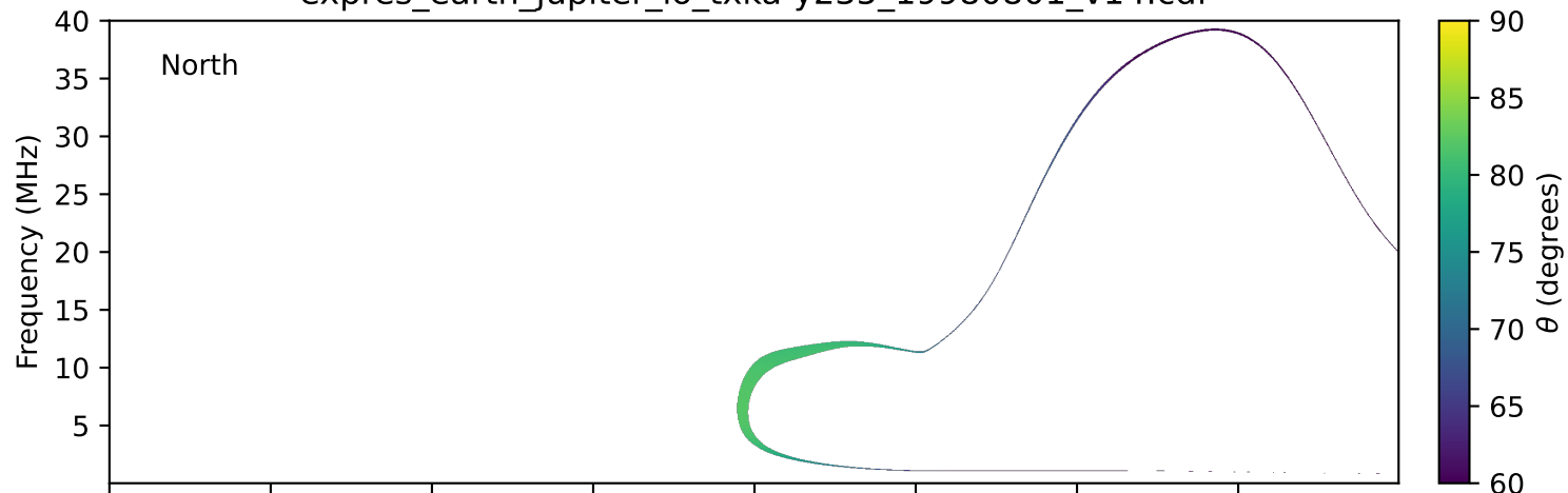
expres_earth_jupiter_io_txka-y235_19980801_v14.cdf
