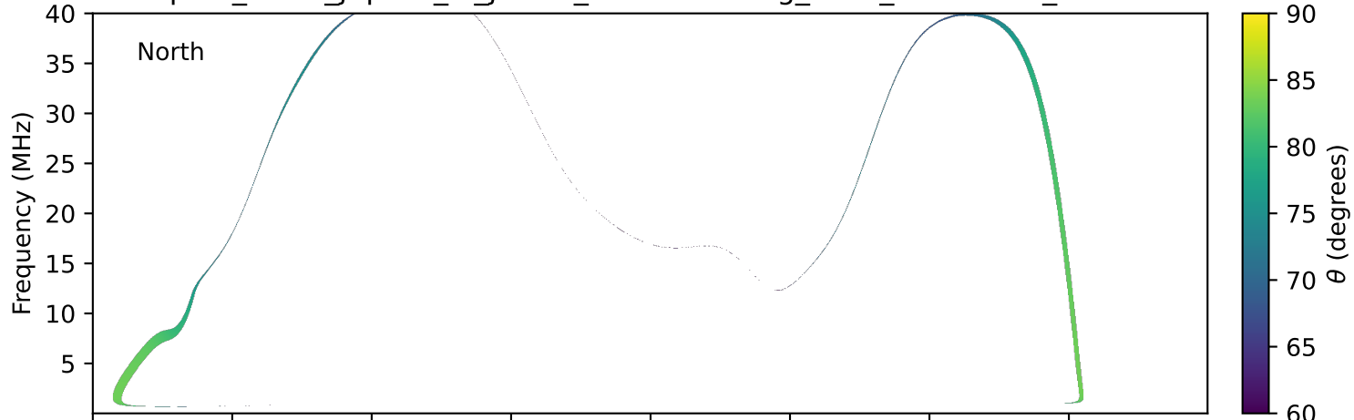
expres_earth_jupiter_io_jrm33_lossc-wid1deg_3kev_19980828_v11.cdf
