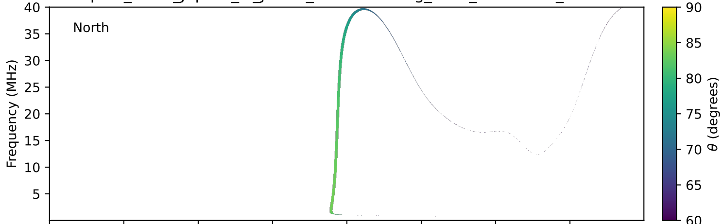
expres_earth_jupiter_io_jrm33_lossc-wid1deg_3kev_19980817_v11.cdf
