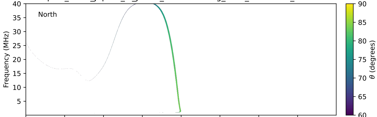
expres_earth_jupiter_io_jrm33_lossc-wid1deg_3kev_19980816_v11.cdf
