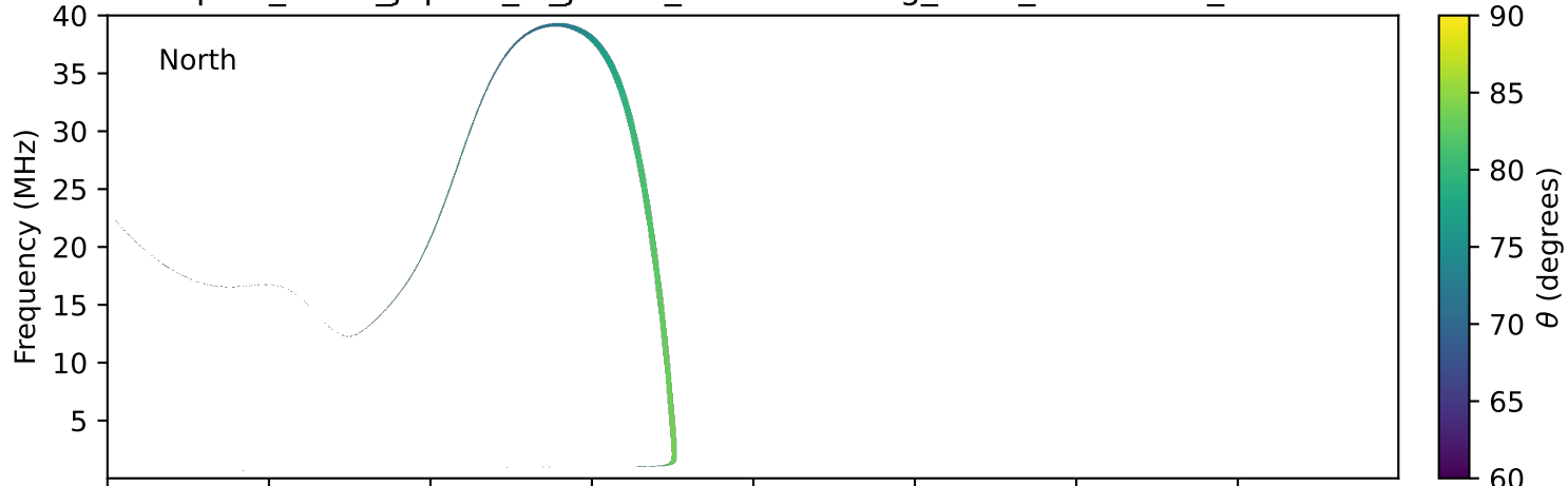
expres_earth_jupiter_io_jrm33_lossc-wid1deg_3kev_19980809_v11.cdf
