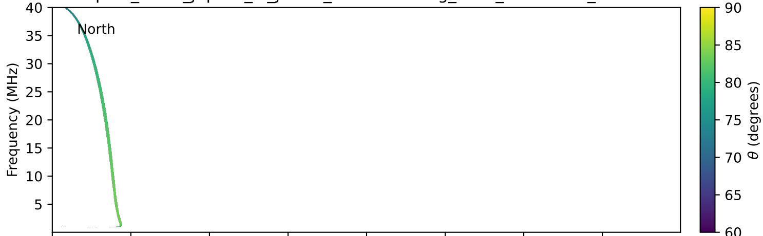
expres_earth_jupiter_io_jrm33_lossc-wid1deg_3kev_19980804_v11.cdf
