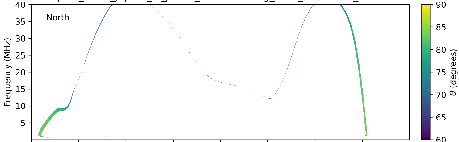
expres_earth_jupiter_io_jrm09_lossc-wid1deg_3kev_19980828_v11.cdf
